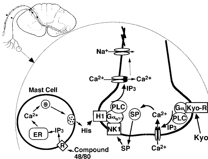
Fig. 8. Schematic model of in vivo signaling in nociceptor endings. The model represents the site of action of Kyo through its receptor, Kyo-R. In the model the nociceptor ending represents SP-containing polymodal C-fiber. It is not yet determined that H1-type His receptor colocalizes with Kyo-R on the same nociceptor ending; however, we have preliminary data showing that His-induced nociception was blocked by i.t. injection of NK1 antagonist (Inoue et al., unpublished data). Details are given in the text. \text{IP}_3 , \text{InsP}_3 ; H1, type 1 His receptor; NK1, neurokinin 1 receptor; R, unidentified receptor; ER, endoplasmic reticulum.
