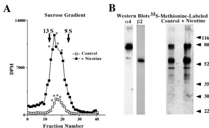
Fig. 8. Purification and separation of fully assembled, [ 35 S]methionine-labeled \alpha 4\beta 2 nAChRs expressed by stably transfected HEK cells. A, sucrose gradients of \alpha 4\beta 2 nAChRs in 2% Triton X-100 extracts from the \alpha 4\beta 2 cell line without and with overnight treatment with nicotine (0.2 μM) were used to isolate fully assembled nAChRs. Extracts for each condition were loaded on 5 to 20% sucrose gradients as described under Materials and Methods . [ 35 S]Methionine-labeled nAChRs were run in parallel. Fractions were collected and then tested on mAb 295-coated microwells with [ 3 H]epibatidine to quantitate nAChRs. The size of T. californica nAChR dimers and monomers are indicated. The location of the peak of the [ 3 H]epibatidine binding was consistent with fully assembled pentameric \alpha 4\beta 2 nAChRs. The four fractions corresponding to the peak (denoted by asterisks) of the gradients were chosen for further immunopurification. These fractions were pooled and nAChRs were isolated with mAb 295-coupled Sepharose. After thorough washing, the isolated nAChRs were eluted with 3% SDS sample buffer and then separated by SDS-PAGE on 10% gels. B, Western blots for \alpha 4 or \beta 2 subunits are shown for the same gel that was used for separation of [ 35 S]methionine-labeled control or nicotine-up-regulated nAChRs. The part of the gel with the [ 35 S]methionine-labeled samples was dried for autoradiography. The bands corresponding to \alpha 4 and \beta 2 subunits were cut from the gels and the amount of 35 S activity was measured by liquid scintillation counting. The values are shown in Table 1.
