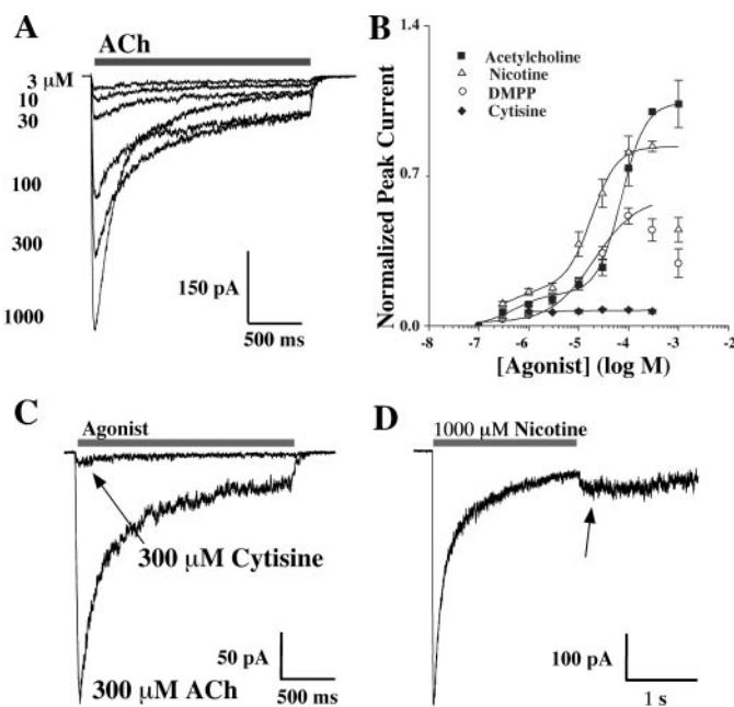
Fig. 1. Pharmacological properties of human \alpha 4\beta 2 nAChRs expressed in HEK cells. A, family of currents recorded in response to increasing concentrations of ACh. B, the concentration/response relationship for \alpha 4\beta 2 nAChRs in HEK cells for ACh, nicotine, DMPP, and cytisine are shown. ACh and nicotine were full agonists, whereas DMPP had about 50% efficacy, and cytisine had 5% efficacy compared with ACh. The EC _{50} values were as follows: DMPP, 20 \pm 2 \mu\text{M} ( n = 4 ); nicotine, 0.3 \pm 0.1 and 18 \pm 2 \mu\text{M} ( n = 4 ); and ACh, 0.7 \pm 0.4 and 74 \pm 6 \mu\text{M} ( n = 7 ). The actual potency of cytisine was obscured by its poor efficacy but seems to be similar to that of nicotine. The responses for nicotine and DMPP that were significantly reduced by secondary properties of the drugs (presumed channel blockade) were excluded from the fits (nicotine at 1 mM and DMPP at 300 \mu\text{M} and 1 mM). C, extremely poor efficacy of cytisine is common to \beta 2 -containing nAChRs (Nelson et al., 2001) and is a hallmark characteristic of \alpha 4\beta 2 nAChRs (Papke and Heinemann, 1994). D, application of high concentrations of nicotine to \alpha 4\beta 2 cell line reveals a sustained rebound current (arrow) that is probably caused by recovery from agonist-mediated channel block. All data were recorded at -60 mV.
