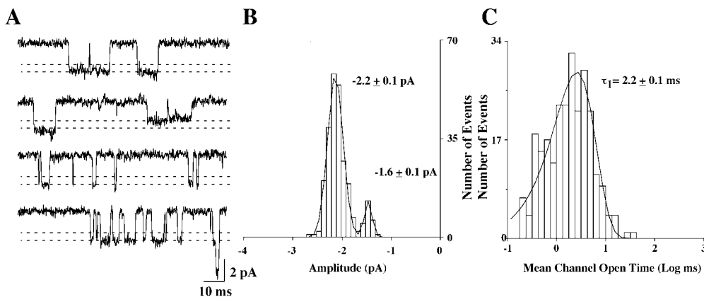
Fig. 6. Single-channel properties of \alpha 4\beta 2 nAChRs after overnight treatment with nicotine. \alpha 4\beta 2 expressing cells were treated overnight with nicotine (5 \mu\text{M} ) before single channel recording. Outside out patches were exposed to equilibrium concentrations of ACh (0.05–10 \mu\text{M} ). A, the representative channel activity was recorded in 500 nM ACh at -80 mV. B, a single conductance-type channel was overwhelmingly present under all conditions. It had a mean amplitude of -2.2 \pm 0.3 pA. Very few openings were observed to a lower conductance level (the amplitude was -1.6 \pm 0.1 pA) regardless of agonist concentration. C, the kinetic behavior of channels recorded after nicotine-treatment was very uniform. Single exponential functions having mean time constants of 2.2 \pm 0.1 ms ( n = 7 ) were most representative of the data. A single patch required an additional component having a time constant of 12 ms.
