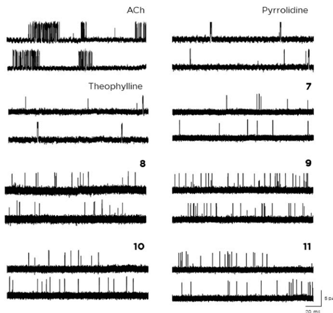
Fig. 2. Activation of the muscle nicotinic acetylcholine receptor by the synthesized caffeine analogs 7–11 . Single-channel events elicited by 30 \mu\text{M} of acetylcholine or 10 \mu\text{M} of pyrrolidine, theophylline, and each compound. Openings were recorded at -70 mV of membrane potential, and they are shown as upward deflections.
