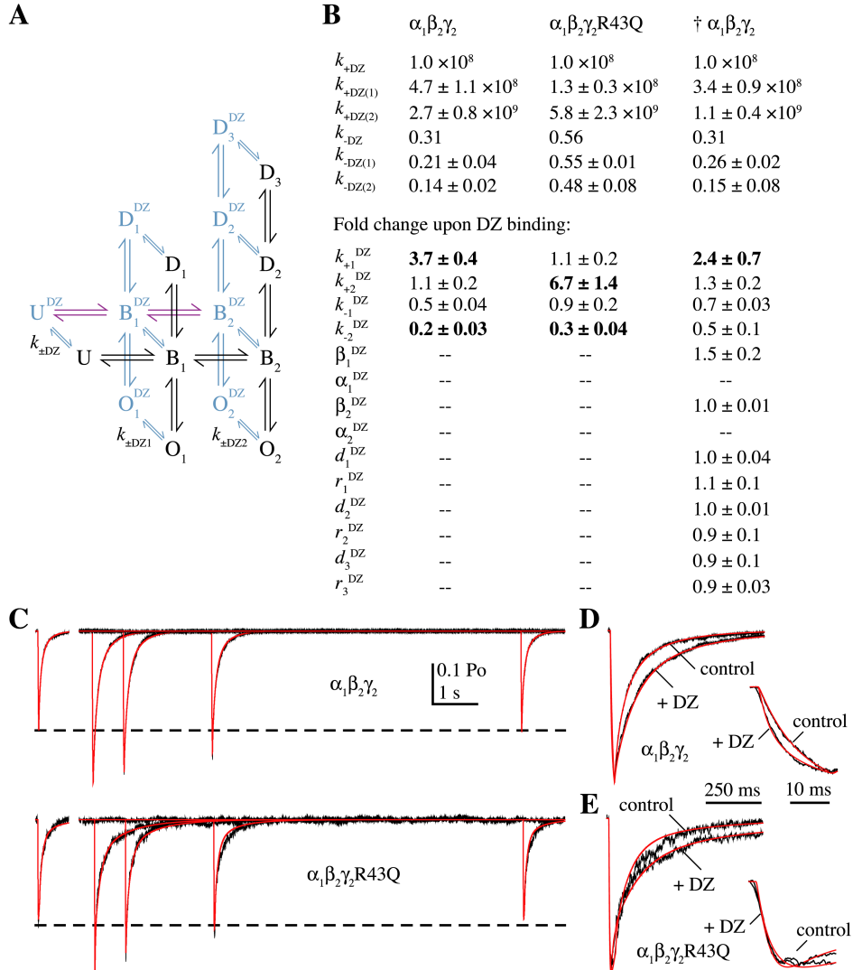
Figure S2: The conclusion that the effects of diazepam (DZ) can be explained by speeding GABA binding and slowing GABA unbinding are unchanged for a model without a loop (compare with Fig. 7 in the main text). A) An extension of the kinetic model shown in figure S1A allowing DZ binding/unbinding from each state (black: DZ-unbound states, blue: DZ-bound states). The rates k_{\pm DZ1} and k_{\pm DZ2} are the same for each set of singly or doubly bound states, respectively, and the rates between DZ-bound states are identical to their DZ-unbound counterparts (transition rates are labeled as in figure S1A) except for the binding and unbinding rates shown in purple, which were allowed to vary (see methods). B) Summary of rate constants or their DZ-induced fold change (mean \pm SEM, bold indicates greater than 2-fold change) for fits to sub-maximal GABA responses alone and following washout of DZ. \dagger Fits were repeated for \alpha_1\beta_2\gamma_2 receptors where all of the DZ-bound rates were allowed to vary except the closing rates \alpha_1 and \alpha_2 as single channel open times are not altered by DZ (Vicini et al., 1987; Rogers et al., 1994). Our overall conclusion that DZ alters GABA binding/unbinding was not changed, and there was also a DZ-induced increase in the singly-bound opening rate constant \beta_1 , suggesting that DZ could have both binding and gating effects. C) Current responses (black) evoked by 20-40 ms pulses of 30 \mu\text{M} GABA alone (offset left) or at varying times following washout of 10 \mu\text{M} DZ (right) for \alpha_1\beta_2\gamma_2 and \alpha_1\beta_2\gamma_2\text{R43Q} receptors overlaid with simulated responses (red). D-E) Expanded view of the fits shown in (C) with the control and maximally potentiated responses overlaid and normalized to illustrate the DZ-induced slowing of deactivation and speeding of the rising phase for \alpha_1\beta_2\gamma_2 receptors (insets).
