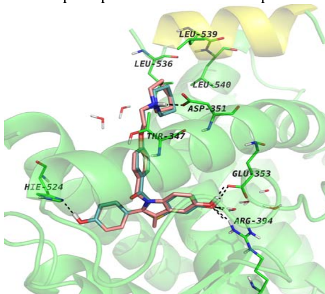
D. BZA superimposed to RAL-ER \alpha complex
