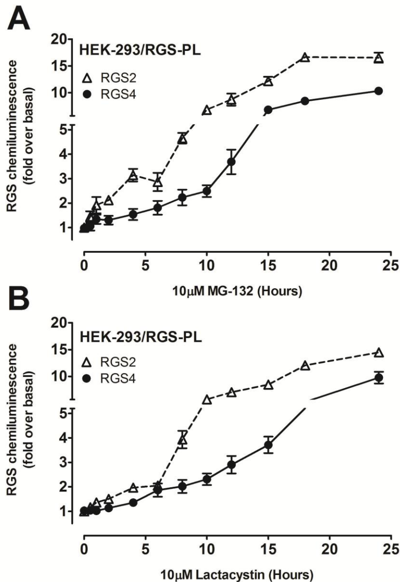
Supplemental figure 1. Time-dependent increase of RGS2 and RGS4 protein expression by proteasome inhibitors. HEK-293 cells stably transfected with RGS2-PL or RGS4-PL were analyzed using the PathHunter™ ProLabel assay. 10μM MG-132 or Lactacystin was added at indicated time points. Both proteasome inhibitors increase both RGS2 and RGS4 protein chemiluminescence in a time-dependent manner. The difference in magnitude between the two proteins could be due to the fact that single clones were used. Results from two experiments run in quadruplicates.
