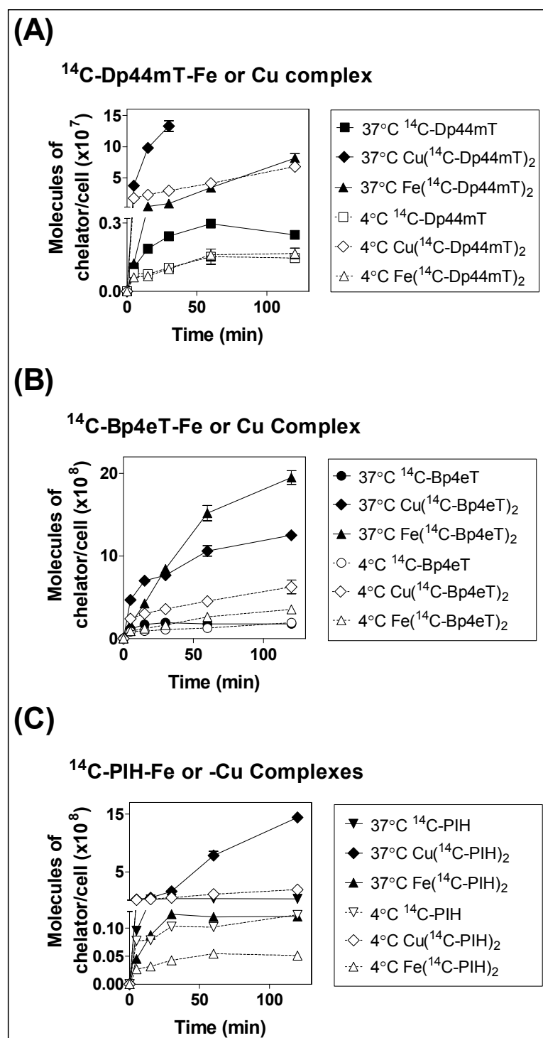
Supplementary Figure 3. The effect of temperature and time on the uptake of the Fe and Cu complexes of ^{14}\text{C} -chelators by SK-N-MC cells. Cells were incubated with media containing (A) ^{14}\text{C} -Dp44mT or its complexes (25 \mu\text{M} ); (B) ^{14}\text{C} -Bp4eT or its complexes (25 \mu\text{M} ); or (C) ^{14}\text{C} -PIH or its complexes (25 \mu\text{M} ) for up to 120 min at 4°C or 37°C. Cells were then washed 4 times on ice with ice-cold PBS and the radioactivity was quantified. Results are mean \pm S.E.M. (3 experiments) and are expressed as molecules of chelator/cell.
