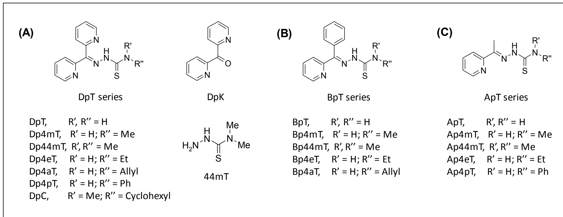
Supplementary Figure 1. Line drawings of the chemical structures of the iron chelators: (A) di-2-pyridylketone thiosemicarbazone (DpT) series; (B) 2-benzoylpyridine thiosemicarbazone (BpT) series; and (C) 2-acetylpyridine thiosemicarbazone (ApT) series. (A) DpT series, namely: DpT, di-2-pyridylketone 4-methyl-3-thiosemicarbazone (Dp4mT), Dp44mT, di-2-pyridylketone 4-ethyl-3-thiosemicarbazone (Dp4eT), di-2-pyridylketone 4-allyl-3-thiosemicarbazone (Dp4aT), di-2-pyridylketone 4-phenyl-3-thiosemicarbazone (Dp4pT) and di-2-pyridylketone 4-cyclohexyl-4-methyl-3-thiosemicarbazone (DpC); Dp44mT precursors (di-2-pyridylketone (DpK) and 4,4-dimethyl-3-thiosemicarbazide (44mT)); (B) the BpT series, namely: BpT, 2-benzoylpyridine 4-methyl-3-thiosemicarbazone (Bp4mT), 2-benzoylpyridine 4,4-dimethyl-3-thiosemicarbazone (Bp44mT), 2-benzoylpyridine 4-ethyl-3-thiosemicarbazone (Bp4eT) and 2-benzoylpyridine 4-allyl-3-thiosemicarbazone (Bp4aT); and (C) the 2-acetylpyridine thiosemicarbazone (ApT) series, namely: ApT, 2-acetylpyridine 4-methyl-3-thiosemicarbazone (Ap4mT), 2-acetylpyridine 4,4-dimethyl-3-thiosemicarbazone (Ap44mT), 2-acetylpyridine 4-ethyl-3-thiosemicarbazone (Ap4eT) and 2-acetylpyridine 4-phenyl-3-thiosemicarbazone (Ap4pT).
