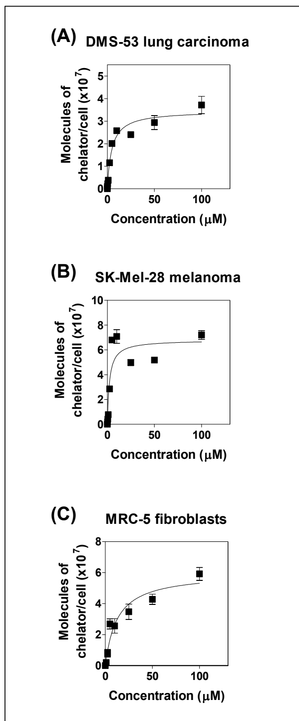
Supplementary Figure 2. The uptake of ^{14}\text{C} -Dp44mT as a function of concentration at 37^\circ\text{C} by: (A) DMS-53 lung carcinoma cells; (B) SK-Mel-28 melanoma cells; and (C) MRC-5 fibroblasts. The cells were incubated in media containing ^{14}\text{C} -Dp44mT (0.1-100 \mu\text{M} ) for 120 min at 37^\circ\text{C} . The cells in Petri dishes were then placed on a tray of ice, washed 4 times using ice-cold PBS, suspended in PBS (1 mL) and the radioactivity was quantified. Results are means \pm S.E.M. of triplicate determinations in a typical experiment.
