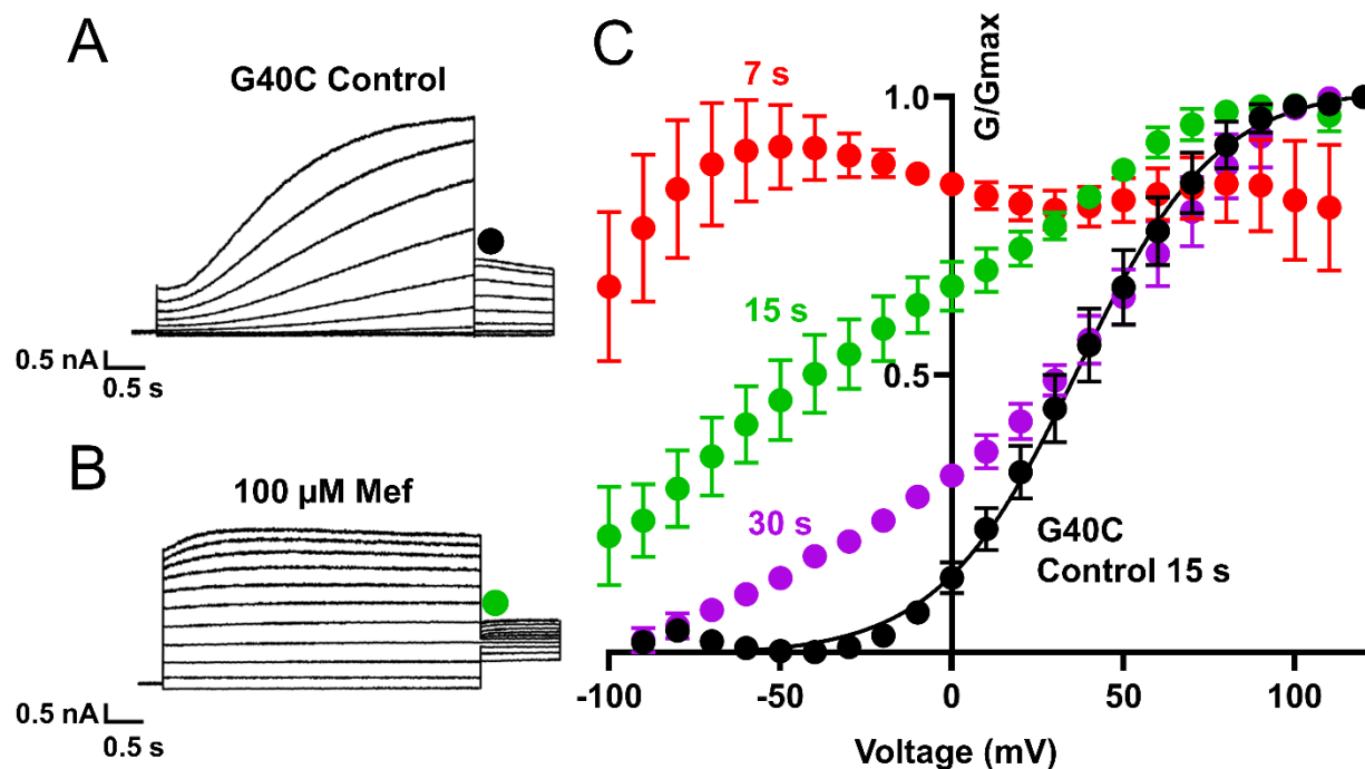
Supplemental Figure 1. Effect of mefenamic acid is preserved in the G40C I_{Ks} mutant. The currents and conductance-voltage (G-V) plots were obtained using the protocols described in Fig. 3. (A) Currents are shown for G40C in the absence of mefenamic acid (control; interpulse interval was 15 s). (B) Currents are shown for G40C in the presence of 100 \mu M mefenamic acid (interpulse interval was 15 s). (C) Effect of different interpulse intervals on G-V plots in control and 100 \mu M mefenamic acid. Intervals were 15 s in control ( n = 4 ; black), and 7 s ( n = 3 ; red), 15 s ( n = 3 ; green) or 30 s ( n = 3 ; purple) in mefenamic acid.
