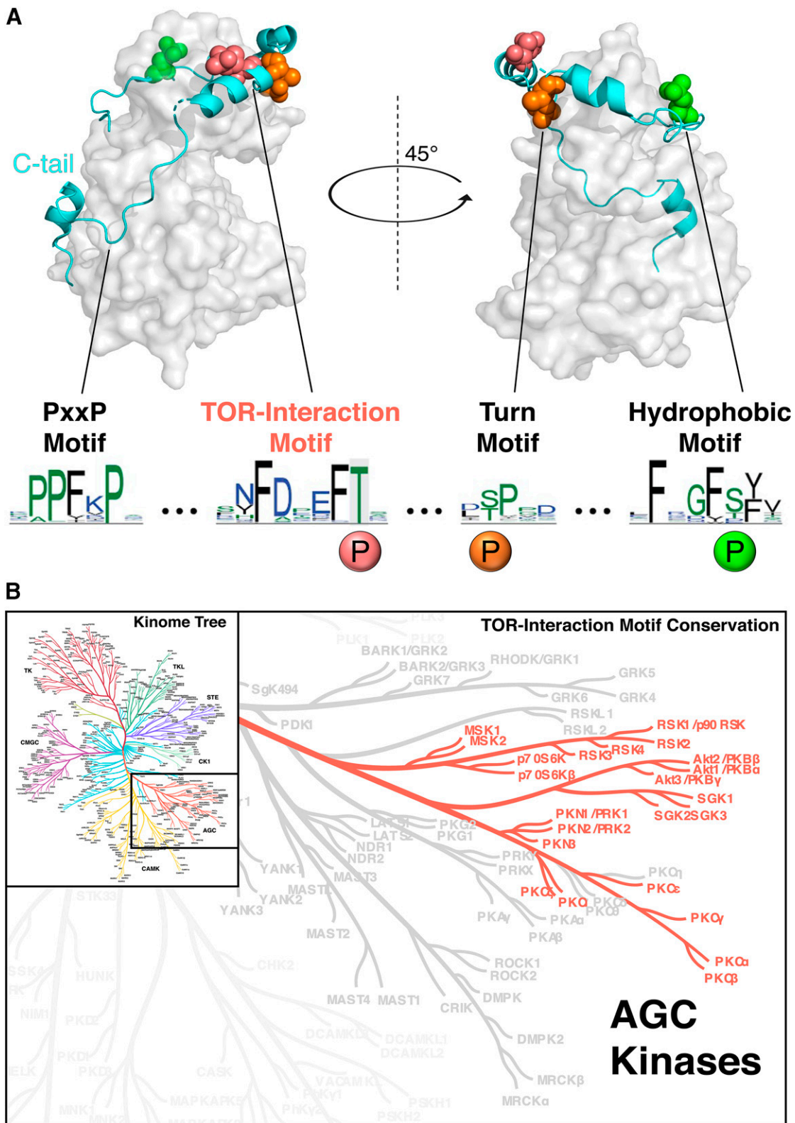
Fig. 1. TIM is a conserved phosphorylation site in mTOR-dependent AGC kinases. (A) Crystal structure of the isolated kinase domain of protein kinase C \beta II (2I0E) showing the conserved C-terminal tail (C-tail; turquoise). The C-tail phosphorylation sites are indicated: TIM (pink; Thr634 in PKC \beta II), turn motif (orange; Thr641 in PKC \beta II), and hydrophobic motif (green; Ser660 in PKC \beta II). Sequence logos display conserved features of the AGC C-tail for all mammalian kinases containing the TIM Thr (F-x3-F-pT), including a conserved PXXP motif (Kannan et al., 2007). (B) AGC branch of the human kinome tree, with red highlighting indicating kinases with the TOR interaction motif (Metz et al., 2018). Adapted from Baffi et al. (2021a). Reprinted with permission from American Association for the Advancement of Science.
