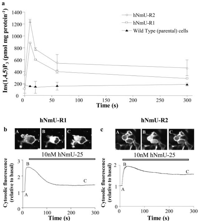
Fig. 3. hNmU-R1- and hNmU-R2-mediated accumulation of \text{Ins}(1,4,5)\text{P}_3 . a, wild-type HEK293 cells ( \blacktriangle ) or cells expressing either hNmU-R1 ( \square ) or hNmU-R2 ( \circ ) were cultured on 24-well plates and challenged with 10 nM hNmU-25 for the time shown before extraction and determination of \text{Ins}(1,4,5)\text{P}_3 using a radioreceptor assay. Data are mean \pm S.E.M., n = 3 . Cells expressing hNmU-R1 (b) or hNmU-R2 (c) were cultured on glass coverslips, transiently transfected with the eGFP- \text{PH}_{\text{PLC}\delta 1} construct, and imaged by confocal microscopy. Cells were challenged with 10 nM hNmU-25 at 15 s. Changes in cytosolic fluorescence [as an index of \text{Ins}(1,4,5)\text{P}_3 levels] were averaged from six cells chosen at random in the field of view but were representative of all cells. Images A, B, and C were taken at the time points indicated on the graphs. Data are representative of at least three separate experiments.
