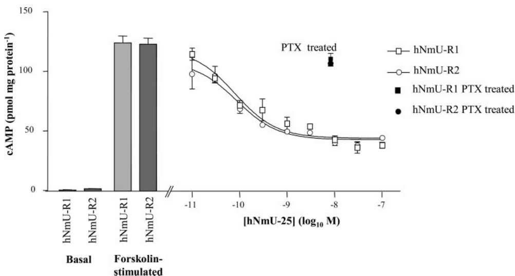
Fig. 5. hNmU-R-mediated inhibition of forskolin-stimulated cAMP accumulation. Cells expressing either hNmU-R1 or hNmU-R2 were cultured on poly-D-lysine-coated 24-well plates. hNmU-25 was added for 10 min before addition of 10 \mu\text{M} forskolin. After a further 10-min incubation, cAMP was extracted and measured by radioreceptor assay. Shown at left are basal and forskolin-stimulated levels of cAMP in cells expressing either hNmU-R1 or hNmU-R2. At right are curves showing the concentration dependence of the hNmU-25-mediated inhibition of forskolin-stimulated cAMP accumulation. The \text{pEC}_{50} values for inhibition were 10.10 \pm 0.16 for hNmU-R1 ( \square ) and 10.06 \pm 0.17 for hNmU-R2 ( \circ ). After pertussis toxin treatment of cells (PTX; 20 h; 100 ng/ml), 10 nM hNmU-25 failed to inhibit forskolin-stimulated cAMP accumulation in cells expressing either hNmU-R1 ( \blacksquare ) or hNmU-R2 ( \bullet ). All data are mean \pm S.E.M., n = 3 .
