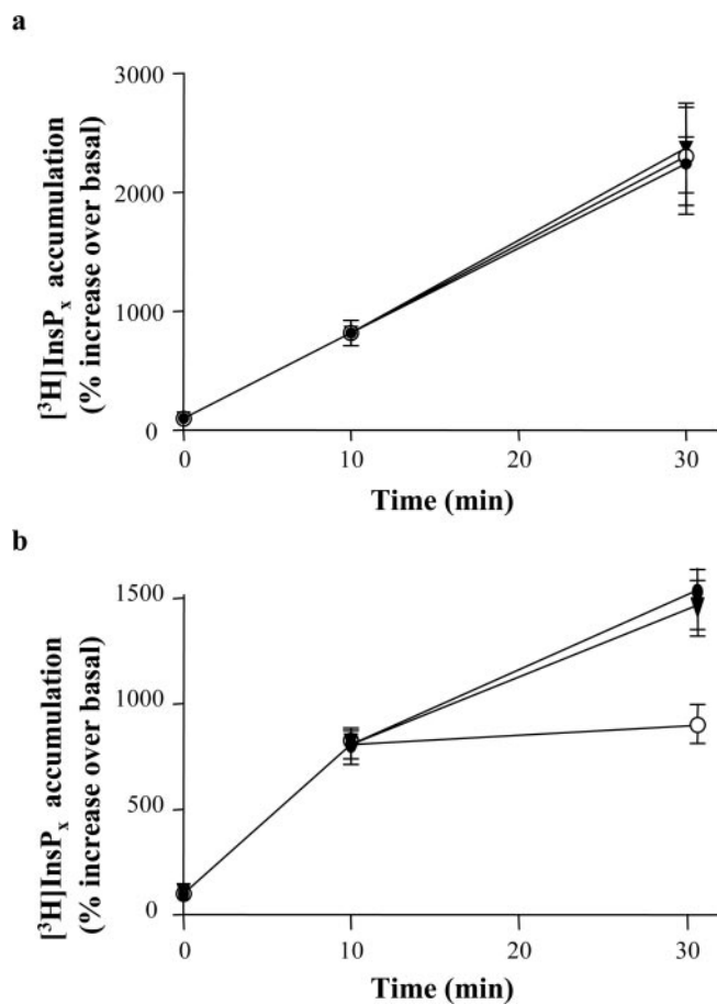
Fig. 9. hNmU-25-mediated accumulation of [ ^3\text{H} ]InsP _x is unaffected by washing to remove extracellular hNmU-25. Wild-type HEK293 cells (b) or cells expressing hNmU-R1 (a) were cultured in 24-well plates and loaded with [ m\gamma - ^3\text{H} ]inositol for 48 h before challenge with 10 nM hNmU-25 in the presence of a 10 mM Li ^+ block of inositol monophosphatase activity. Cells were challenged with 10 nM hNmU-25 (a) or 100 \mu\text{M} carbachol (b) and after 10 min were either untreated (●) or the buffer removed and the cells washed (three times with 1 ml of buffer) before replacement of buffer either without (○) or with (▼) agonist. Data are mean \pm S.E.M., n = 3 .
