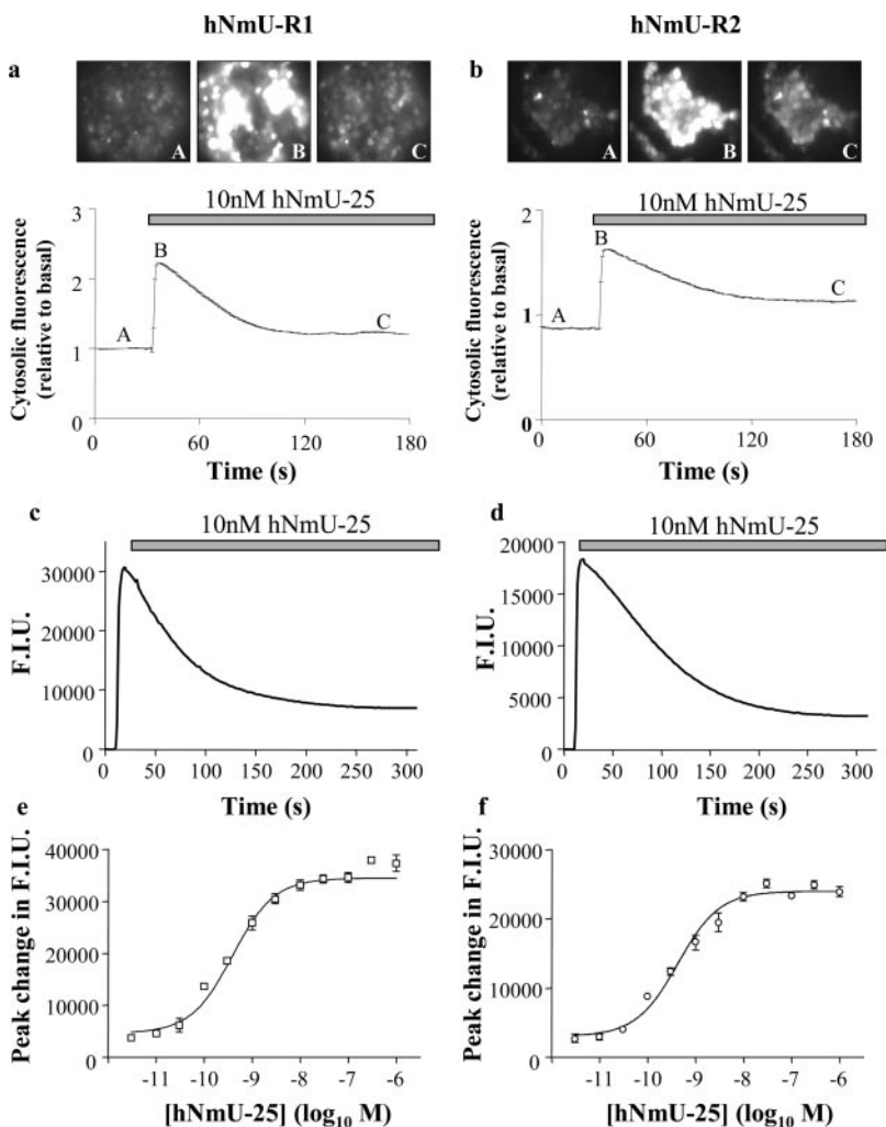
Fig. 4. hNmU-R1- and hNmU-R2-mediated changes in [\text{Ca}^{2+}]_i . hNmU-R1- (a) or hNmU-R2- (b)-expressing cells were cultured on glass coverslips, loaded with fluo-3-AM, and cytosolic fluorescence was determined by confocal microscopy as an index of [\text{Ca}^{2+}]_i . Cells were challenged with 10 nM hNmU-25 at 30 s. Traces show the average change in cytosolic fluorescence of six cells in the field of view chosen at random. Images A, B and C were taken at the time points indicated on the traces. Data are representative of at least four separate experiments. c to f, [\text{Ca}^{2+}]_i in cell populations was determined using fluo-4-loaded cells and a FLIPR. The time course of 10 nM hNmU-25-mediated changes in fluorescence intensity units (F.I.U.) as an index of [\text{Ca}^{2+}]_i is shown for cells expressing either hNmU-R1 (c) or hNmU-R2 (d). The concentration-response relationships for hNmU-25-mediated peak elevations of [\text{Ca}^{2+}]_i in cells expressing either hNmU-R1 (e) or hNmU-R2 (f) gave \text{pEC}_{50} values of 9.41 \pm 0.09 and 9.37 \pm 0.06 , respectively. Data are mean \pm S.E.M., n = 3 .
