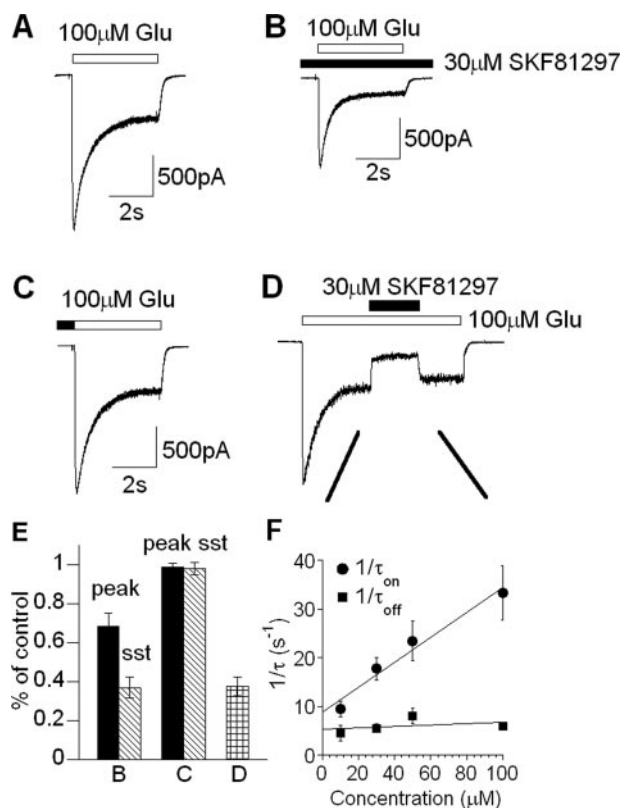
Fig. 1. Effects of the D1 agonist SKF81297 on NMDA receptor (NR1A/NR2A) mediated currents. A, control response to 100 \mu\text{M} glutamate. B, 30 \mu\text{M} SKF81297 (black bar) significantly inhibited the NMDA receptor-mediated current. C, no inhibition was detected when SKF81297 was only applied before the glutamate application. D, significant inhibition was observed when SKF81297 was applied 2 s after the receptor activation. E, summary of percentages of the current amplitude changes in B, C, and D. Changes in peak and steady state (sst) current amplitudes were measured. F, the inverse of time constants of SKF81297 block, derived from single exponential fits of onset and recovery process, were plotted against the SKF81297 concentration. 20 \mu\text{M} glycine was included in all glutamate-containing solutions. Error bars represent S.E.
