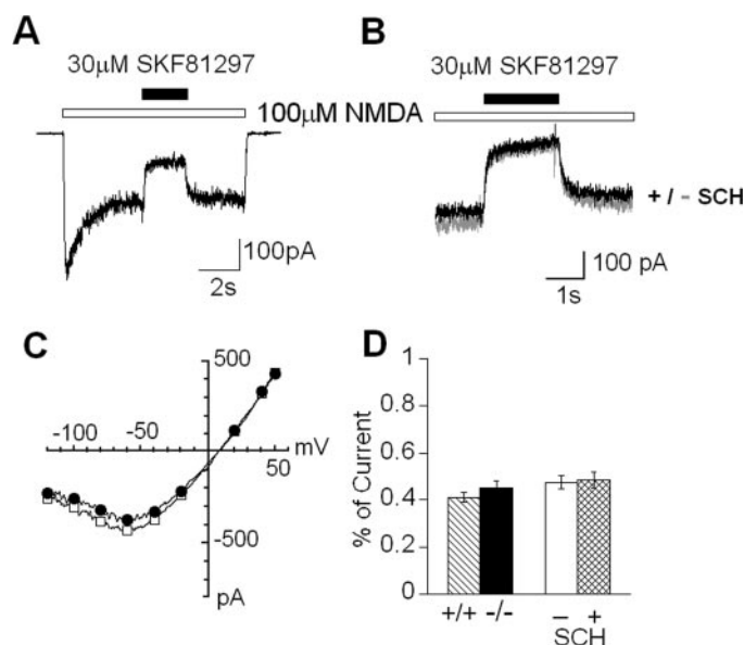
Fig. 5. Effects of SKF81297 on NMDA receptor-mediated currents in neurons. A, 30 \mu\text{M} SKF81297 significantly blocked NMDA receptor-mediated current from a medium spiny neuron acutely isolated from D1 receptor knockout mouse. B, using 0.5 \mu\text{M} SCH23390, a D1 receptor antagonist, to detect the D1 receptor-independent effect of SKF81297. The black trace is obtained in the presence of 0.5 \mu\text{M} SCH23390. C, I-V relationship of effects of SKF81297 with and without the presence of 0.5 \mu\text{M} SCH23390. The \bullet and \square represent with and without 0.5 \mu\text{M} SCH23390. D, comparing blocking effects of 30 \mu\text{M} SKF81297 using medium spiny neurons isolated from wild type (+/+) and D1 receptor knockout (-/-) mice; and hippocampal neurons with or without 0.5 \mu\text{M} SCH23390.
