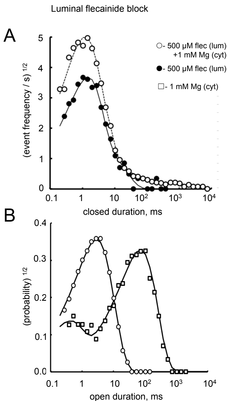
Supplemental Figure. Dwell-time analysis of luminal flecainide inhibition. (A) Closed dwell-time histograms showing the rate of closed events based on the method of Sigworth and Sine (1987) as described in the text. (B) Corresponding open dwell-time histograms. The legend applies to A and B.
