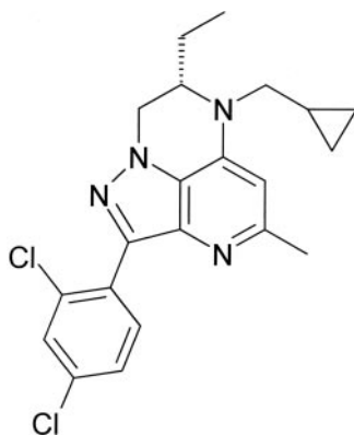
NBI 35965 [( S )-6-cyclopropylmethyl-2-(2,4-dichlorophenyl)-7-ethyl-4-methyl-7,8-dihydro-6 H -1,3,6,8 a -tetraaza-acenaphthylene mesylate].
