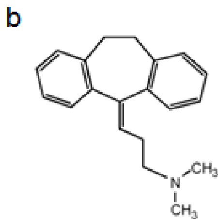
Amitriptyline structure
